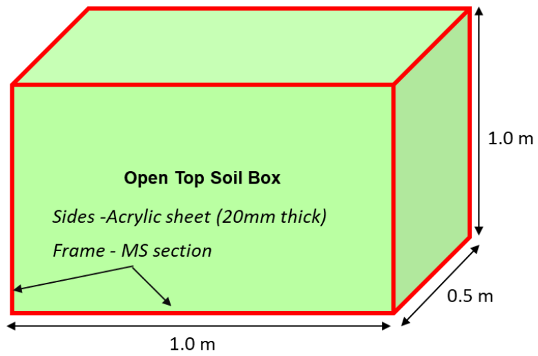
Figure 5. Open Top Soil Box [size - 1.0m(L) x 1.0m(H) x 0.5m(W)]
