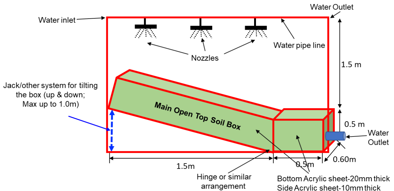
Figure 4. Tilting Soil box (Open Top)
