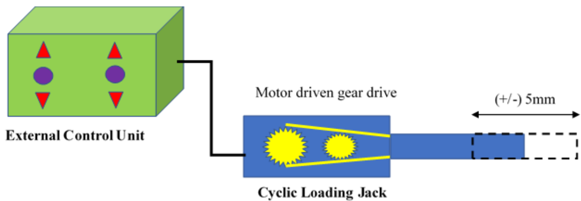
Figure 1. Cyclic Loading Jack with Servo Cylinder
