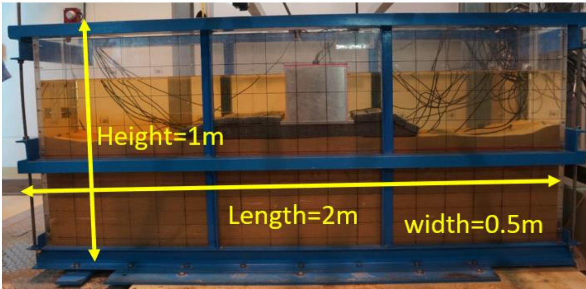
Figure 2. Soil box (this picture is for indication purpose only. Please ignore soils and model inside the soil box)
