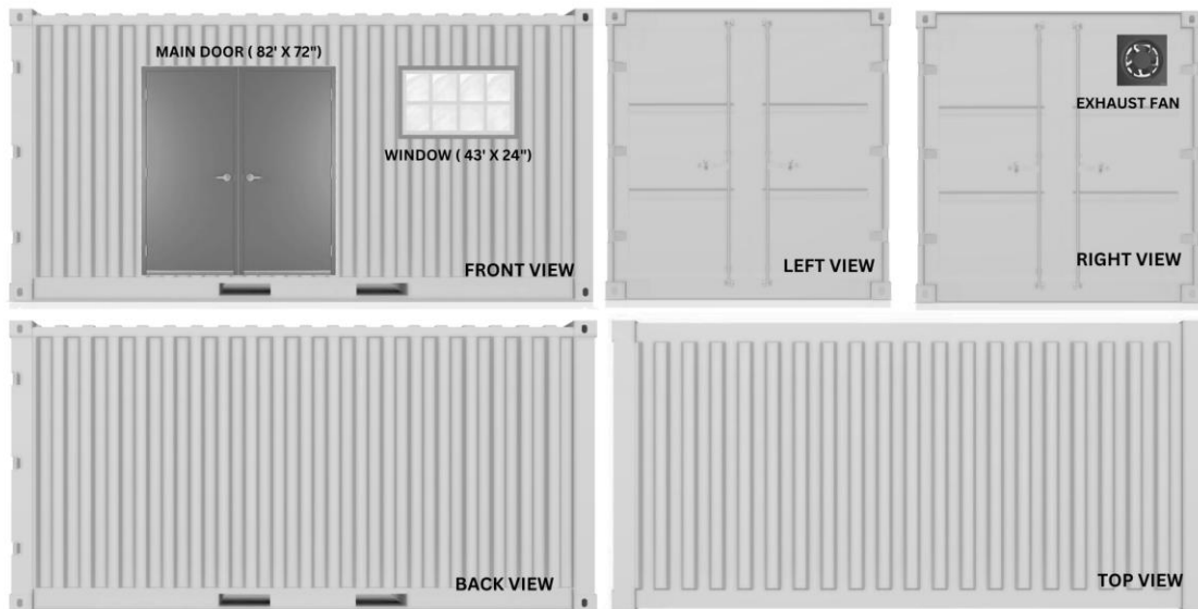
STANDARD SHIPPING CONATINER : LENGTH X BREADTH X HEIGHT = 20' X 8' X 8'
